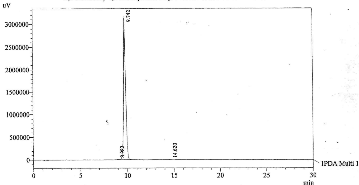
Chromatogram 2,6-Dimethoxy-1,4-benzoquinone D:\promonence\Data\2013\AUG-2013\160813F.lcd
